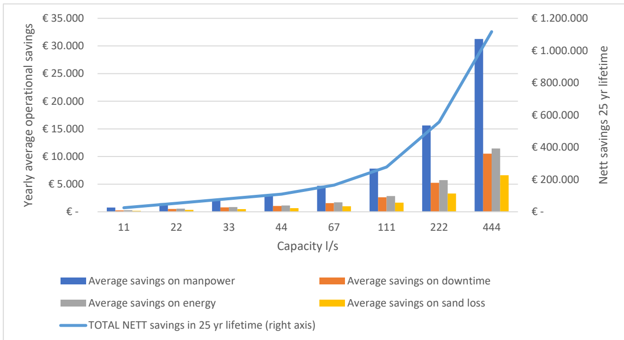
Figure 5 Estimated savings per parameter for 8 plant sizes based on their capacity (l/s).
